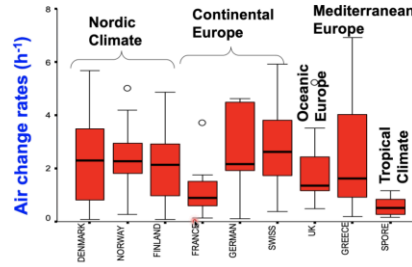
Air change rates (ACH) measured in the European and Singapore buildings studied
