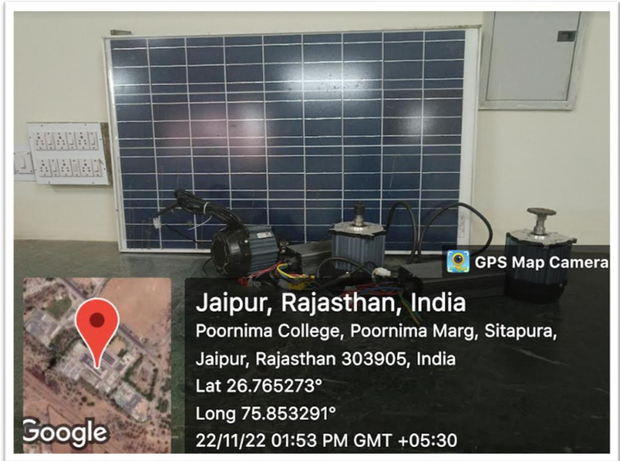
Solar Energy based Experimental Setup
